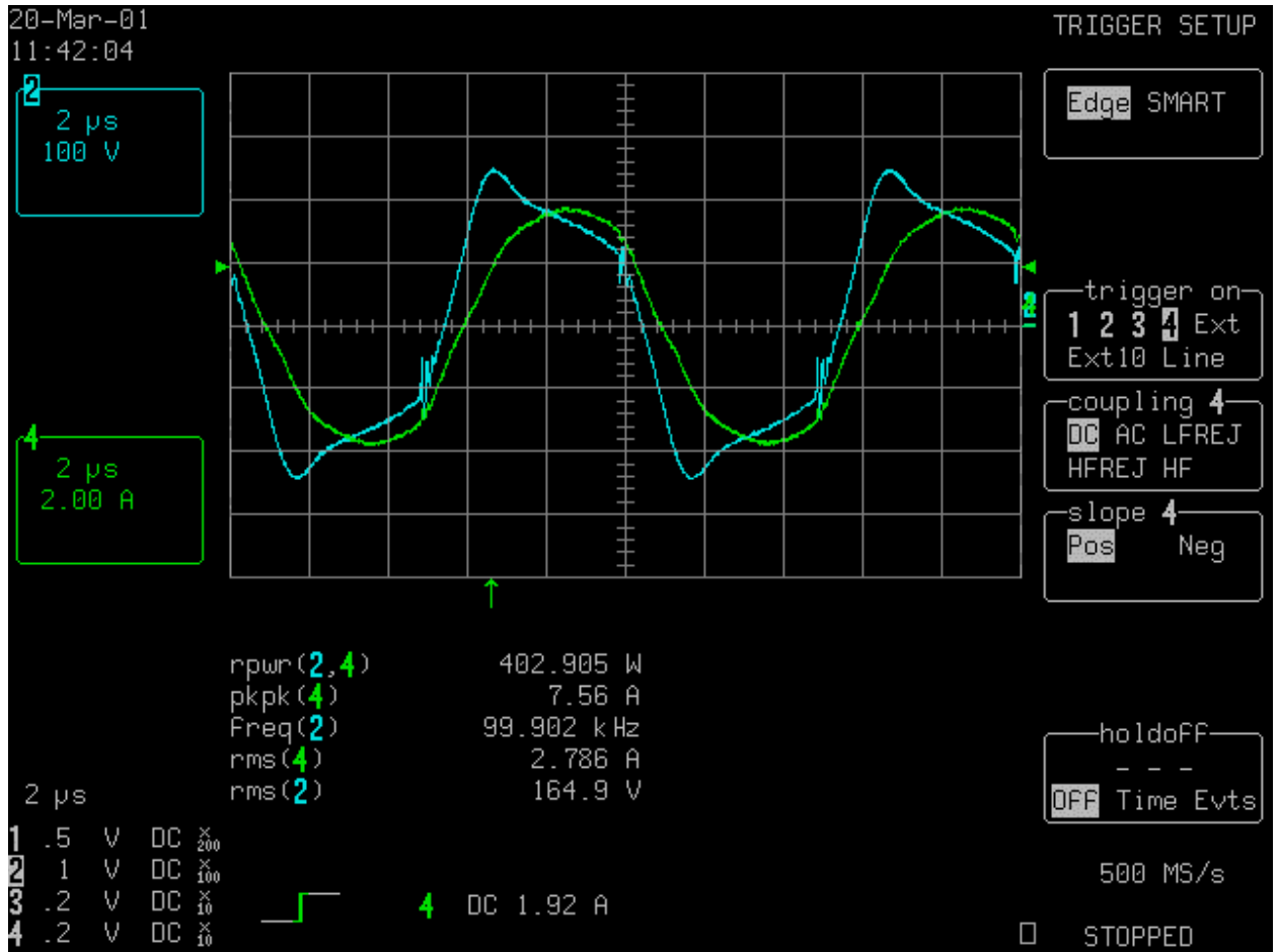
Fig. 3 With airflow Ch 2 - Voltage, Ch 4 - Current
